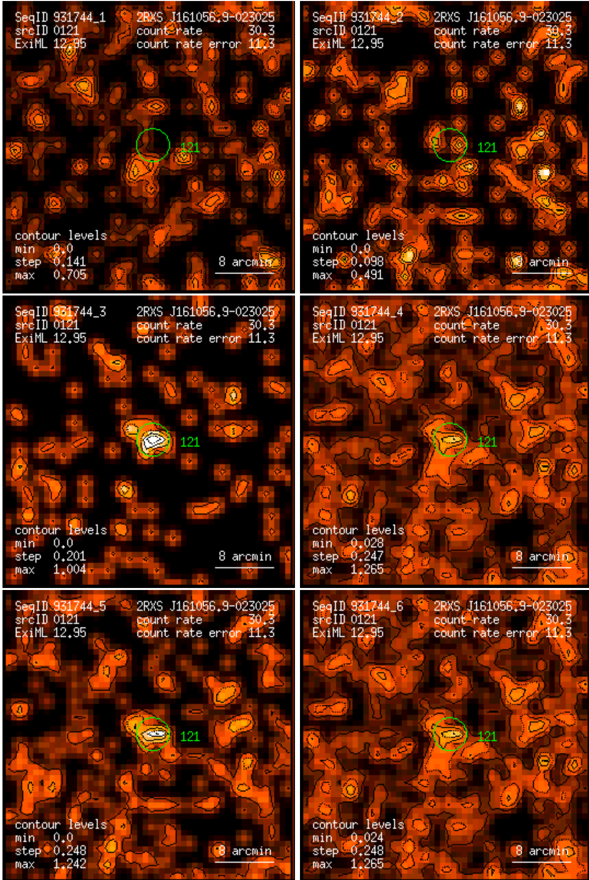
Figure 121: RASS 931744: detection 0121: band rate images, Gaussian filter: (1) PSPC channels 11 – 41, (2) 52 – 90, (3) 91 – 201, (4) 11 – 235, (5) 52 – 201, (6) 11 – 201. Broad band rates in counts/ks. Band rate contour levels in counts/ks/arcmin 2 .
