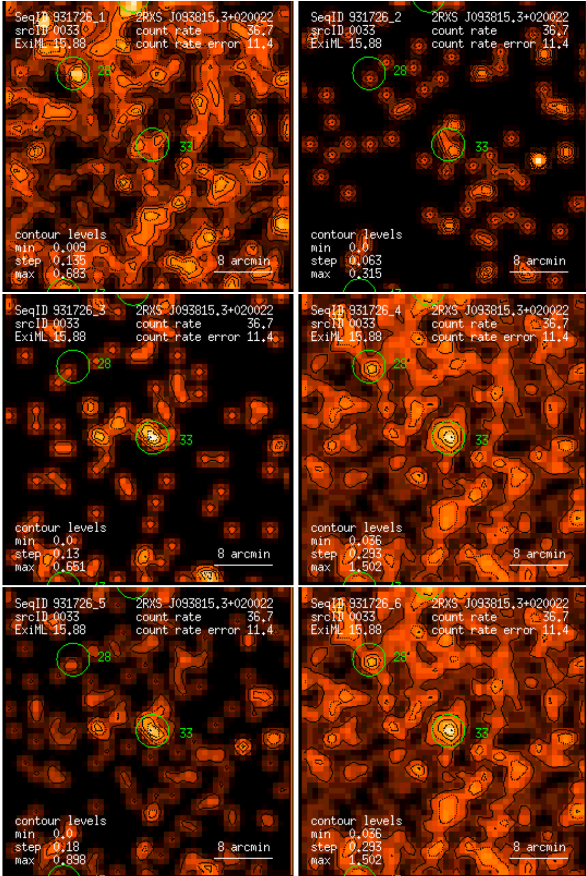
Figure 33: RASS 931726: detection 0033: band rate images, Gaussian filter: (1) PSPC channels 11 – 41, (2) 52 – 90, (3) 91 – 201, (4) 11 – 235, (5) 52 – 201, (6) 11 – 201. Broad band rates in counts/ks. Band rate contour levels in counts/ks/arcmin 2 .
