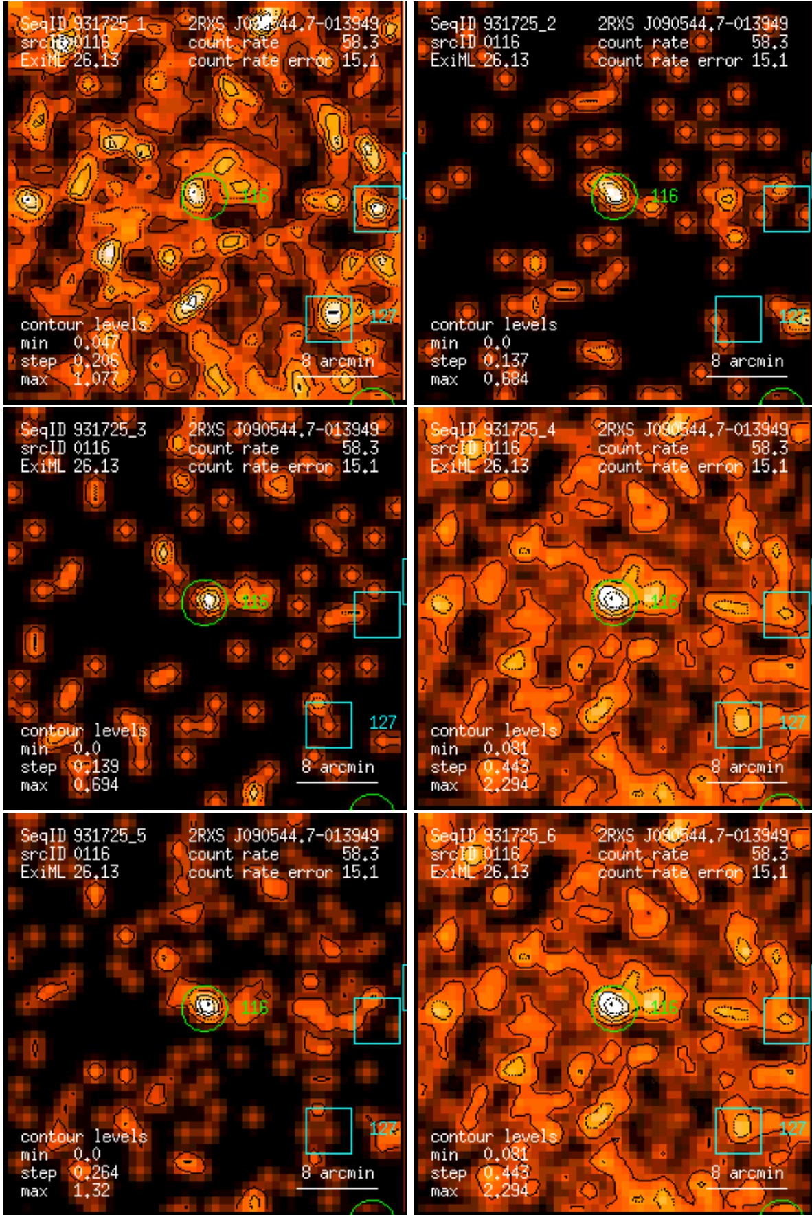
Figure 116: RASS 931725: detection 0116: band rate images, Gaussian filter: (1) PSPC channels 11 – 41, (2) 52 – 90, (3) 91 – 201, (4) 11 – 235, (5) 52 – 201, (6) 11 – 201. Broad band rates in counts/ks. Band rate contour levels in counts/ks/arcmin 2 .
