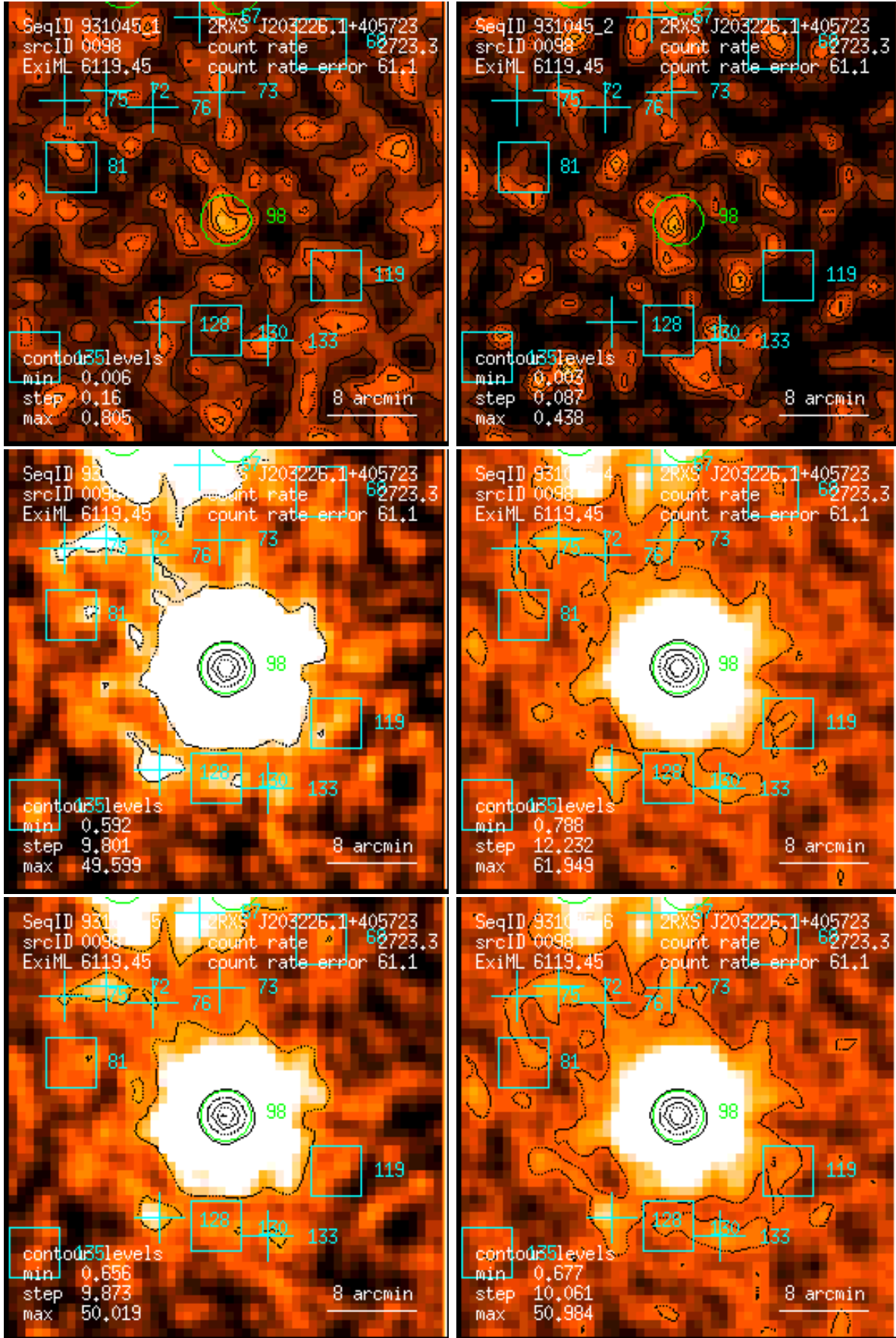
Figure 98: RASS 931045: detection 0098: band rate images, Gaussian filter: (1) PSPC channels 11 – 41, (2) 52 – 90, (3) 91 – 201, (4) 11 – 235, (5) 52 – 201, (6) 11 – 201. Broad band rates in counts/ks. Band rate contour levels in counts/ks/arcmin 2 .
