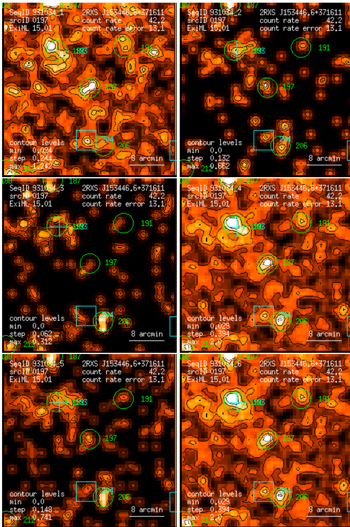
Figure 197: RASS 931034: detection 0197: band rate images, Gaussian filter: (1) PSPC channels 11 – 41, (2) 52 – 90, (3) 91 – 201, (4) 11 – 235, (5) 52 – 201, (6) 11 – 201. Broad band rates in counts/ks. Band rate contour levels in counts/ks/arcmin 2 .
