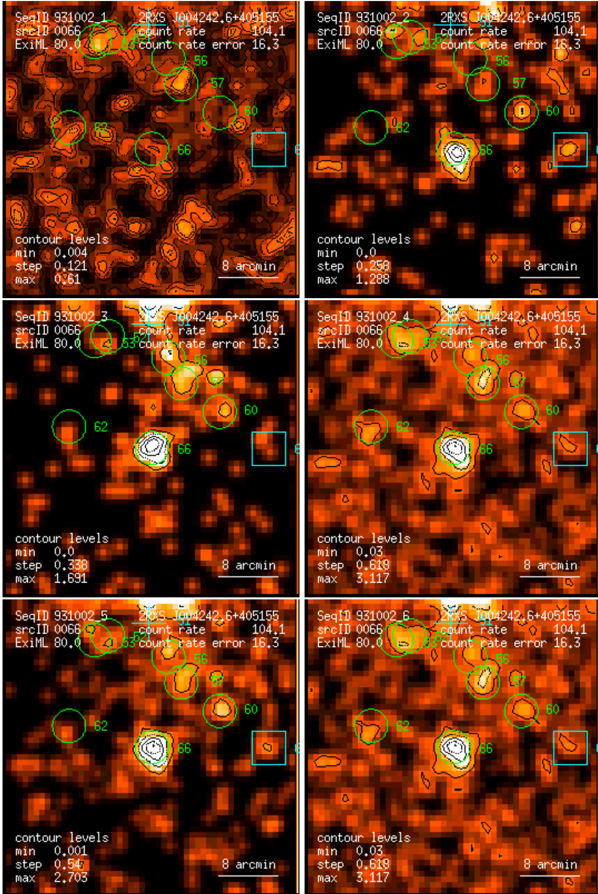
Figure 66: RASS 931002: detection 0066: band rate images, Gaussian filter: (1) PSPC channels 11 – 41, (2) 52 – 90, (3) 91 – 201, (4) 11 – 235, (5) 52 – 201, (6) 11 – 201. Broad band rates in counts/ks. Band rate contour levels in counts/ks/arcmin 2 .
