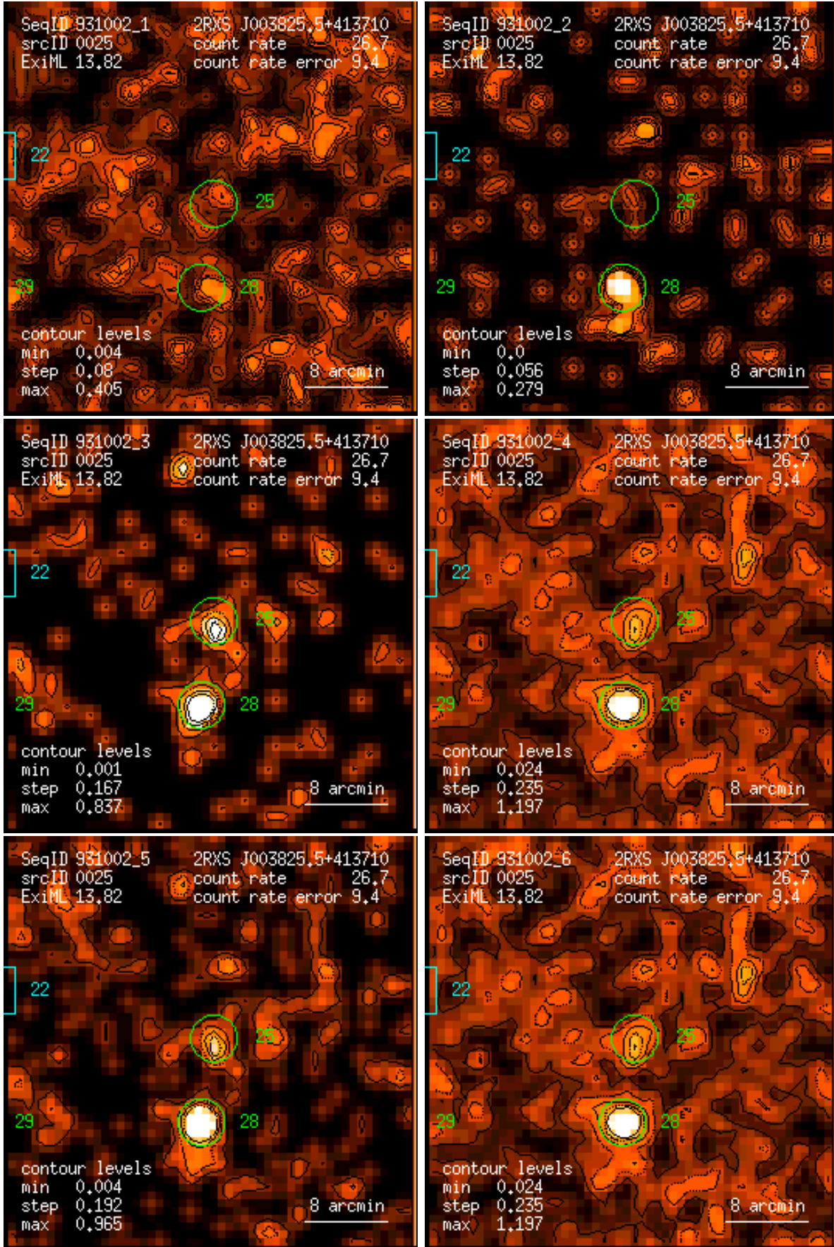
Figure 25: RASS 931002: detection 0025: band rate images, Gaussian filter: (1) PSPC channels 11 – 41, (2) 52 – 90, (3) 91 – 201, (4) 11 – 235, (5) 52 – 201, (6) 11 – 201. Broad band rates in counts/ks. Band rate contour levels in counts/ks/arcmin 2 .
